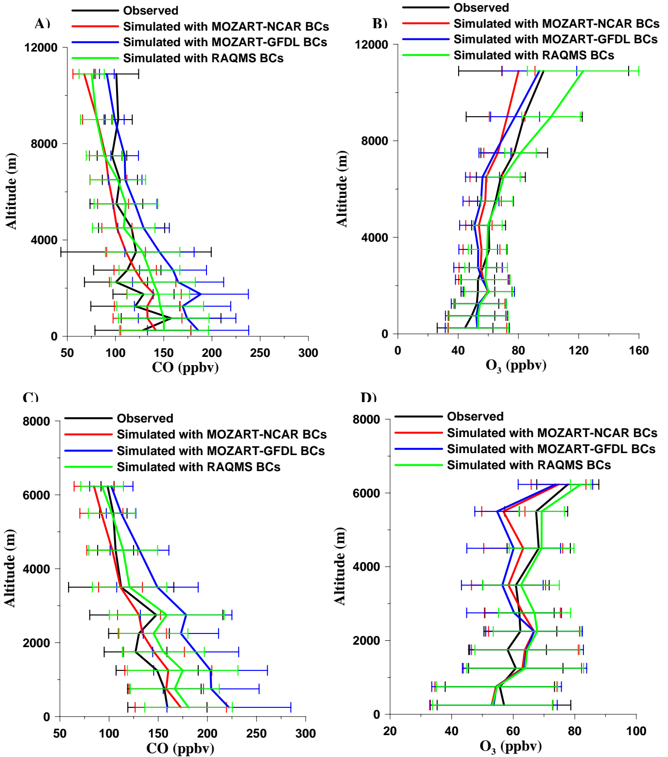
Figure 10. Observed and 60km-simulated CO and O 3 mean profiles and standard deviations for all DC-8 flights (A, B) and WP-3 flights (C, D)
