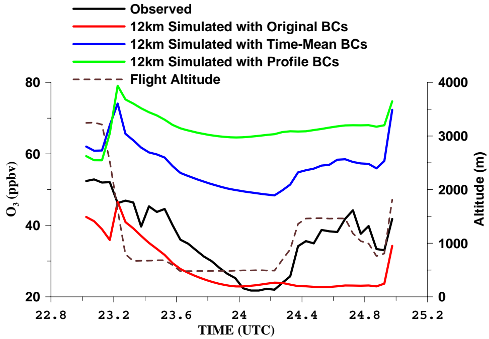
Figure 8. Observed and simulated CO and O 3 concentrations for the WP-3 flight 13 on 07/31- 08/01, 2004
