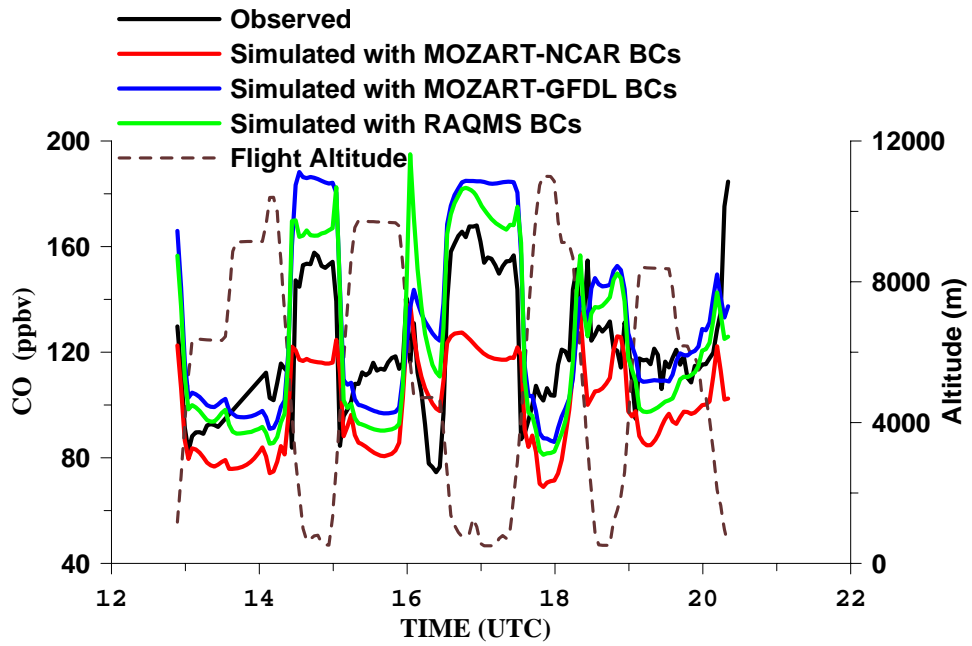
Figure 6. Observed and Simulated O 3 and CO concentrations for the DC-8 flight 8 on 07/15/2004
