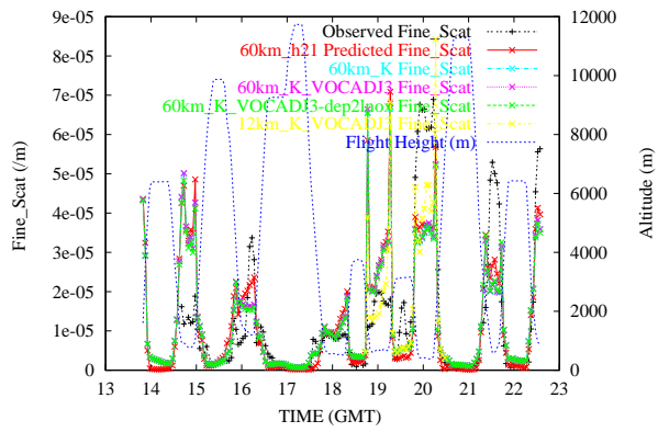
ICARTT DC-8 Flight #5 Fine_Scat on 7/8/2004
