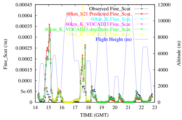
ICARTT DC-8 Flight #6 Fine_Scat on 7/10/2004
